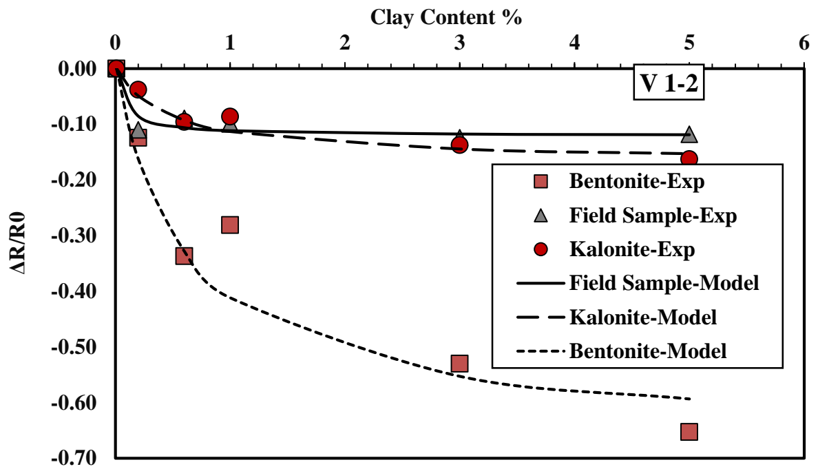
Figure 7 Testing and Modeling the Variation of Vertical Resistance with the Addition of Clay
