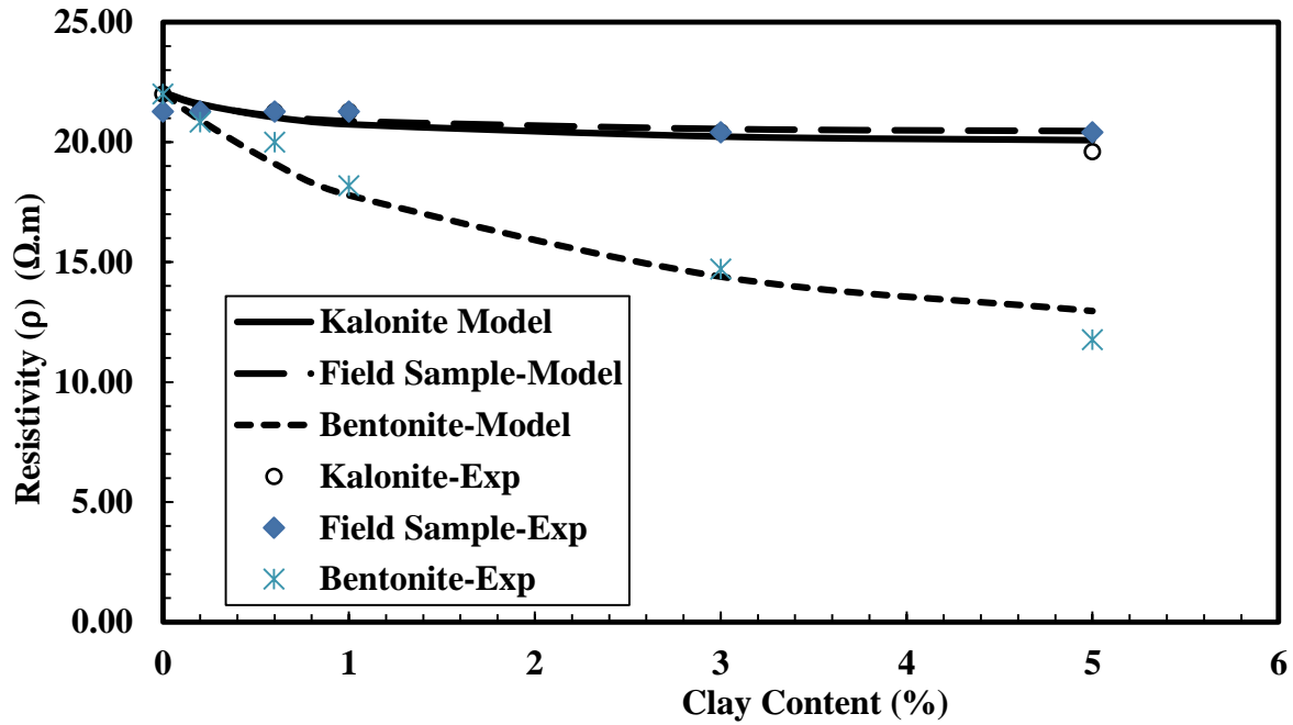
Figure 6 Testing and Modeling the Variation of Vertical Resistivity with the Addition of Clay
