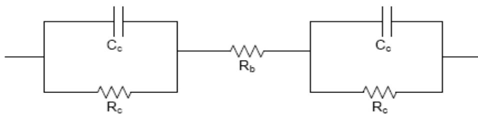
Figure 3. Equivalent Circuit for the Two-Probe CASE-2
