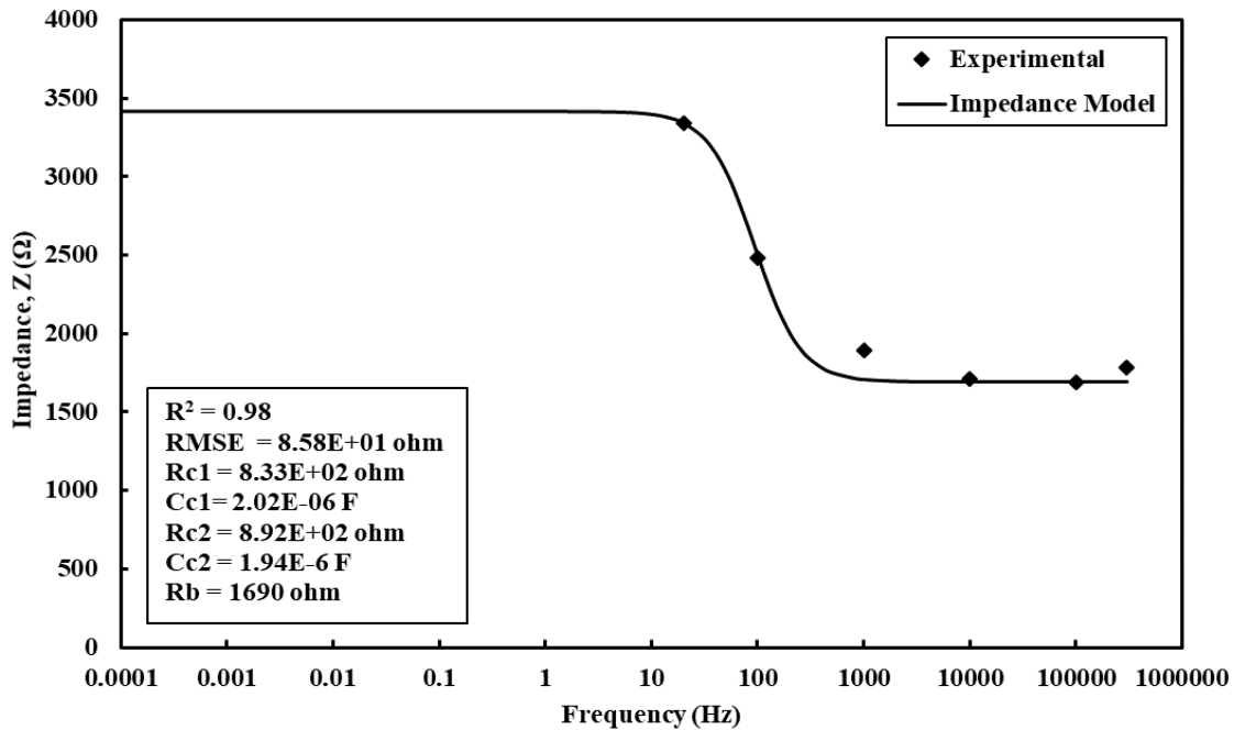
Figure 5 Typical Impedance-Frequency Response of Water contaminated with 2.5% Bentonite Clay
