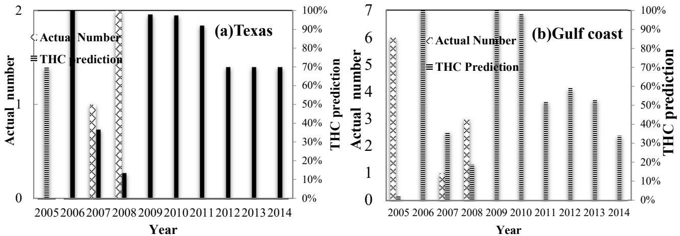
Figure 1 Actual Hurricanes and Probability Predicted by THC for the past decade (a) Texas and (b) U.S. Gulf Coast
