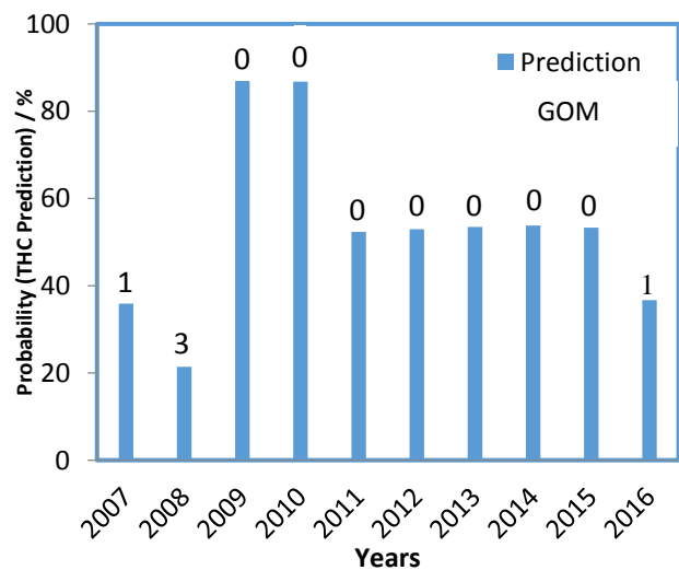
Figure 1: Actual Hurricanes and Probability Predicted by THC for the past decade (a) Texas and (b) U.S. Gulf Coast
